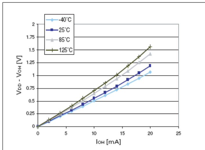
Figure 35: Typ. V_{DD} - V_{OH} @ V_{DD} = 5 V (high sink ports)
