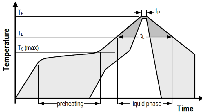
Figure 14 Soldering profile according to JEDEC standard. Recommended conditions are T_P = 245\text{ }^{\circ}\text{C} and t_P \leq 30\text{ sec} for Pb-free assembly, T_L < 220\text{ }^{\circ}\text{C} and t_L < 150\text{ s} . Ramp-up rate < 3\text{ }^{\circ}\text{C/s} and ramp-down rate < 4\text{ }^{\circ}\text{C/s} .
