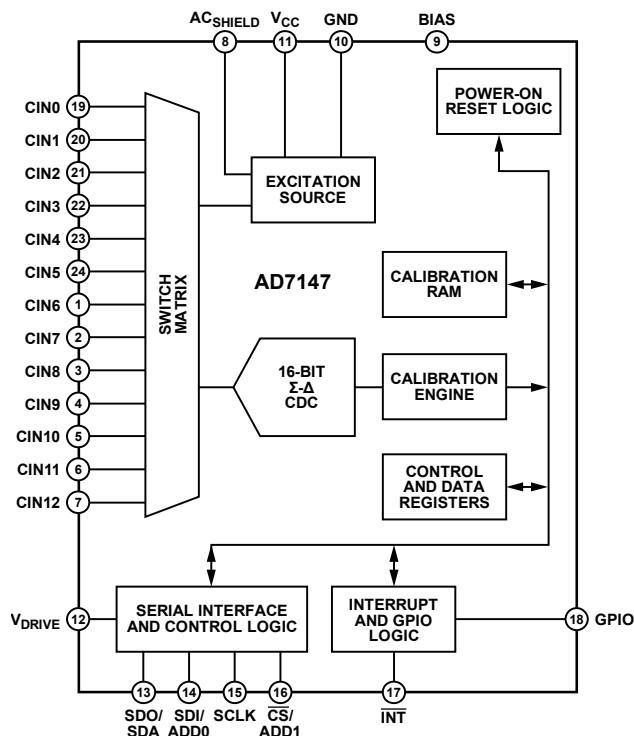
Figure 1. AD7147 Block Diagram
