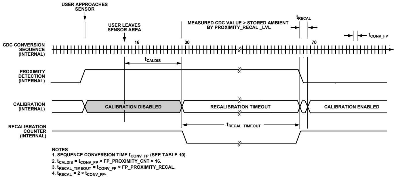
Figure 31. Example of Full Power Mode Proximity Detection with Forced Recalibration (FP_PROXIMITY_CNT = 1 and FP_PROXIMITY_REC = 40)
