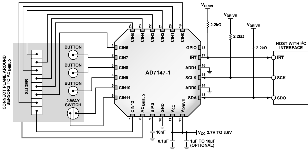
Figure 60. Typical Application Circuit with I²C Interface
