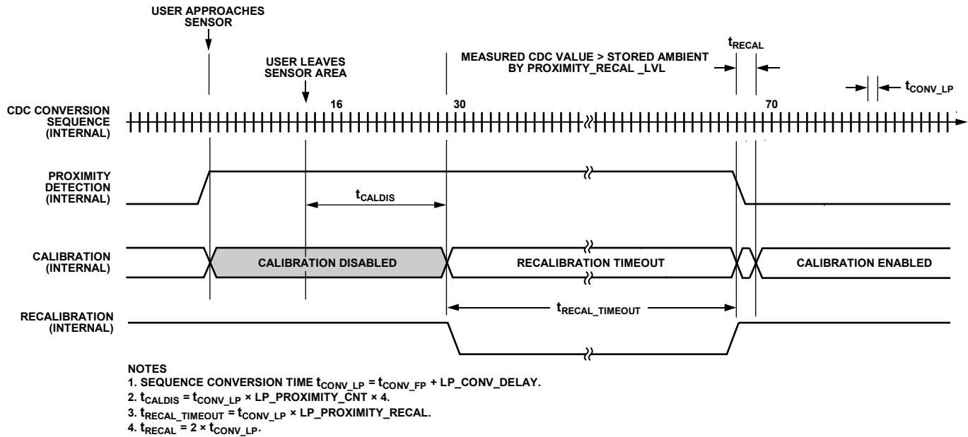
Figure 32. Example of Low Power Mode Proximity Detection with Forced Recalibration (LP_PROXIMITY_CNT = 4 and LP_PROXIMITY_REC = 40)
