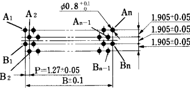
(26, 34, 50 contacts)
