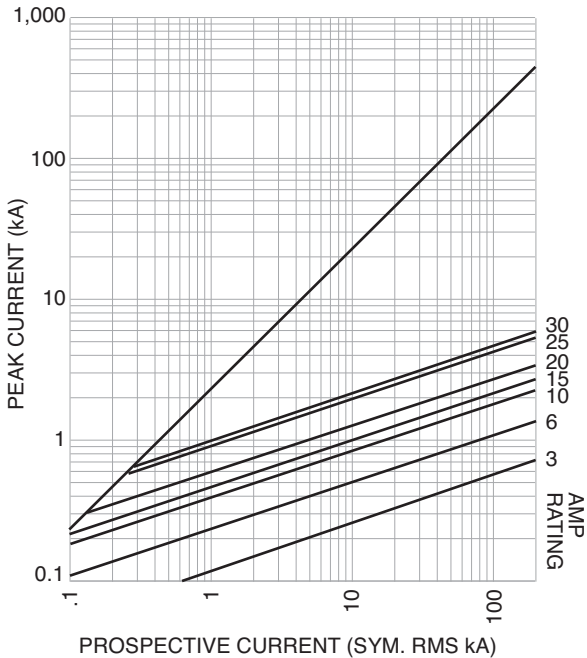
Peak Let-Through Curves (Cat. No. CIF21)
