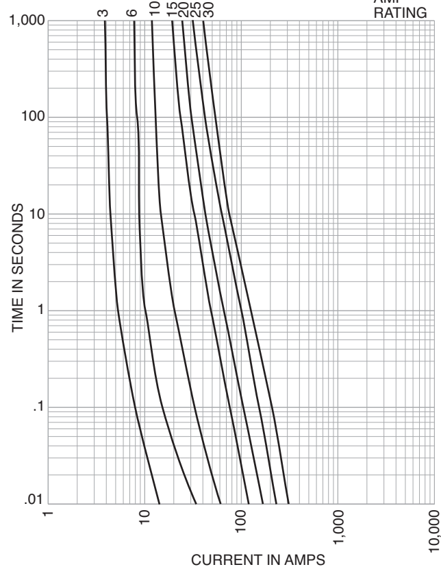
Time-Current-Curves (Cat. No. CIF21)
