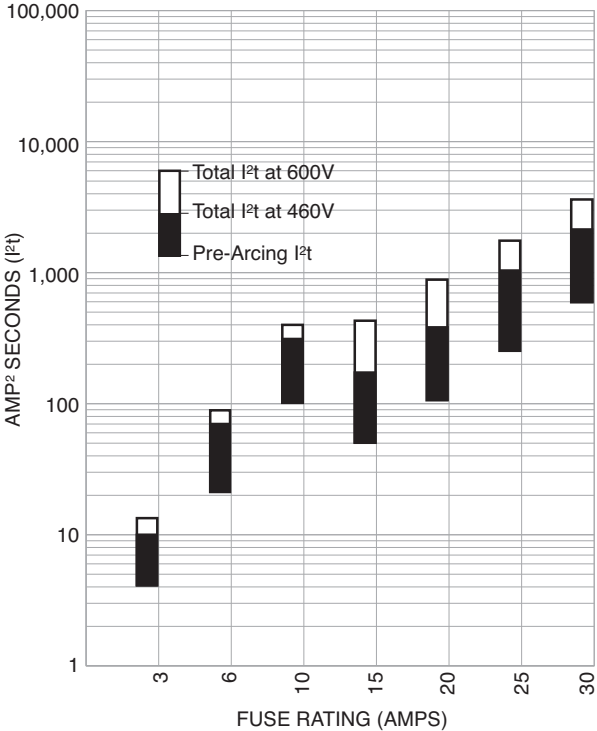
Energy Let-Through Curves (Cat. No. CIF21)
