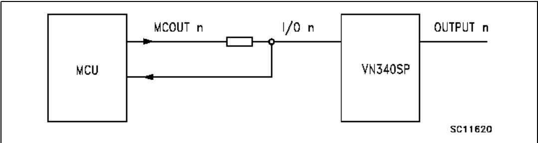
Figure 9. Driving circuit
