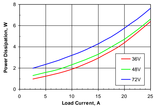
Figure 4. Power dissipation vs. load current and input voltage for SSQE48T25015 converter mounted vertically with air flowing from pin 1 to pin 3 at a rate of 300 LFM (1.5 m/s) and T_a = 25^{\circ}C .
