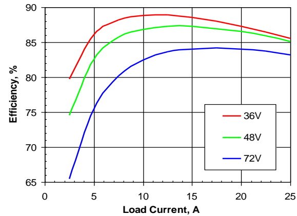
Figure 2. Efficiency vs. load current and input voltage for SSQE48T25015 converter mounted vertically with air flowing from pin 1 to pin 3 at a rate of 300 LFM (1.5 m/s) and T_a=25^{\circ}C .
