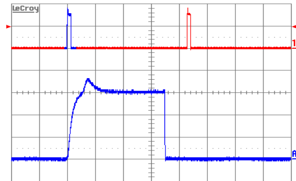
Figure 15. Load current (top trace, 20 A/div., 50 ms/div.) into a 10 m\Omega short circuit during restart, at V_{in} = 48 V. Bottom trace (10 A/div., 2 ms/div.) is an expansion of the on-time portion of the top trace.
