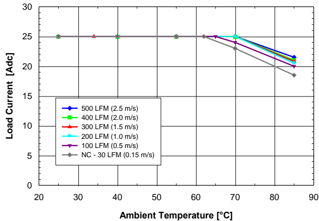
Figure 1. Available load current vs. ambient air temperature and airflow rates for SSQE48T25015 converter mounted vertically with air flowing from pin 1 to pin 3, V_{in} = 48V . Note: NC – Natural convection
