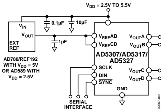
Figure 41. AD5307/AD5317/AD5327 Using a 2.5 V External Reference
