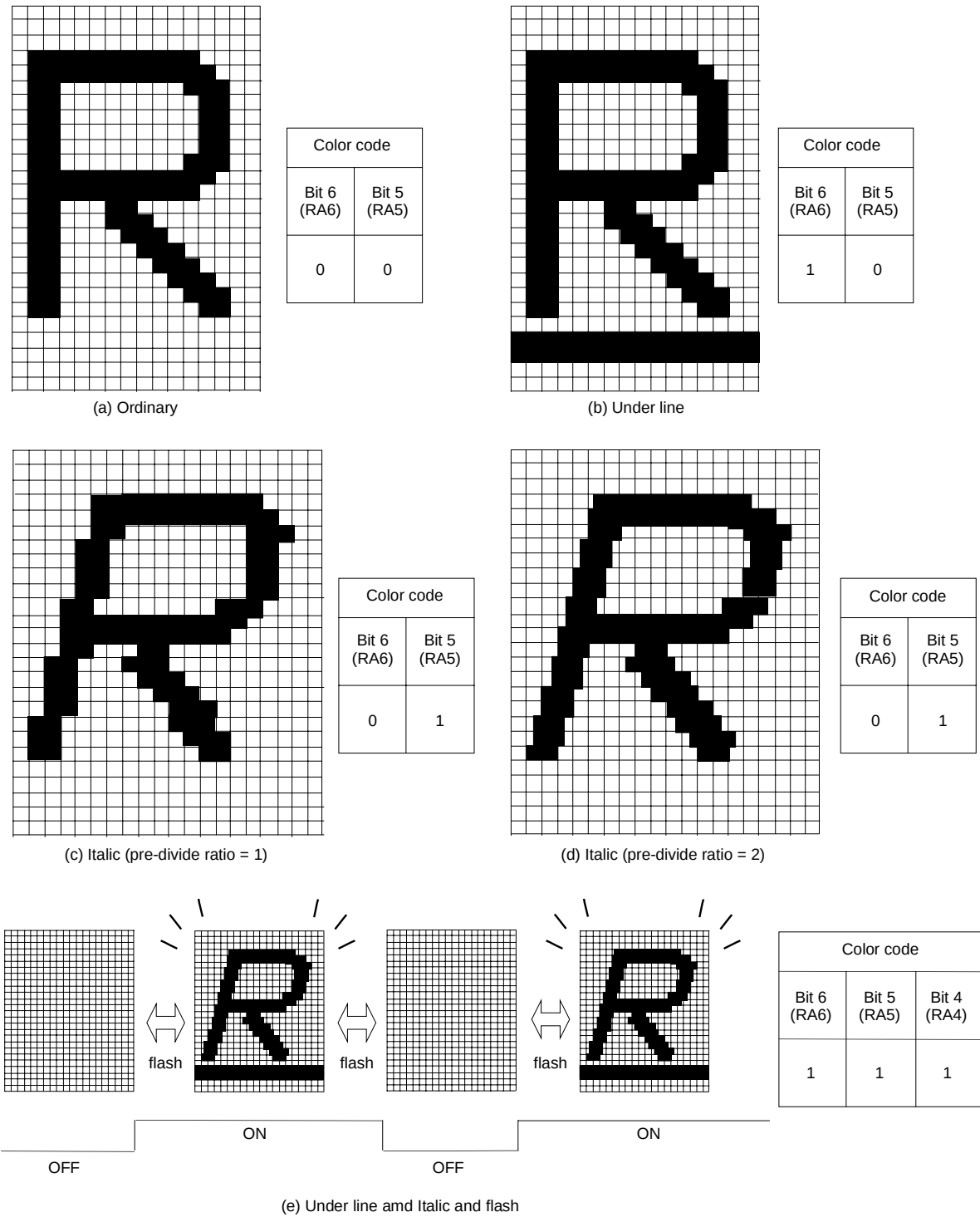
Fig. 8.11.18 Example of Attribute Display (in CC Mode)
