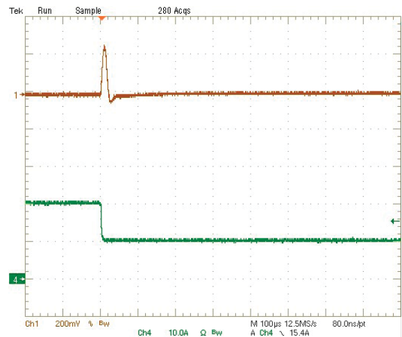
Step Load Transient Response (Vin=5V, Vout=0.6V, Cload=94µF, Iout=20A to 10A) Trace 1=Vout, 200 mV/div, Trace 4=Iout, 10A/div.
