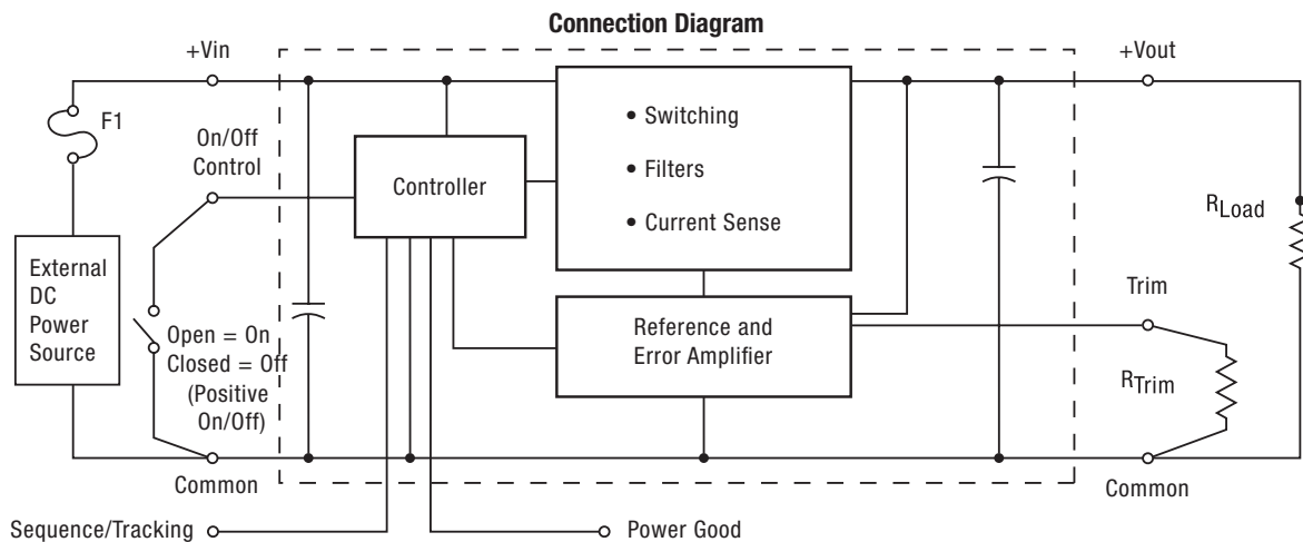
Figure 1. OKL2-T/20-W5
