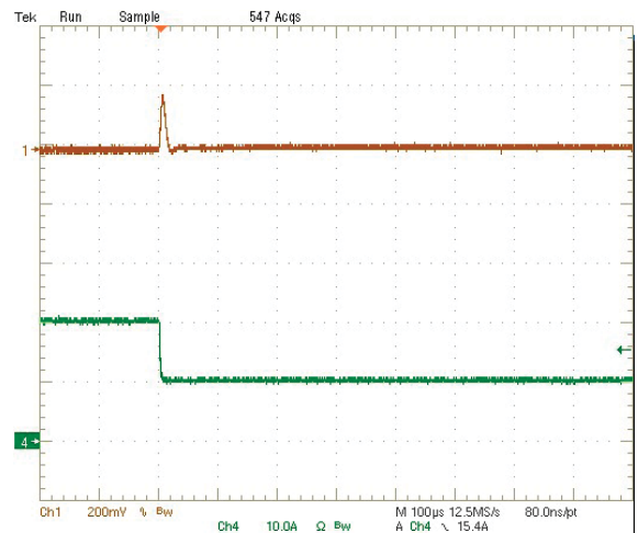
Step Load Transient Response (Vin=5.0V, Vout=2.5V, Cload=94µF, Iout=20A to 10A) Trace 1=Vout, 200 mV/div, Trace 4=Iout, 10A/div.
