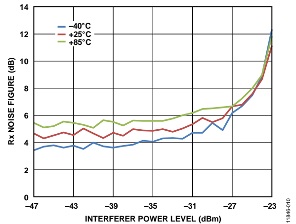
Figure 10. Rx Noise Figure vs. Interferer Power Level, EDGE Signal of Interest with P_{IN} = -90 dBm, CW Blocker at 3 MHz Offset, Gain Index = 64
