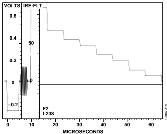
NOISE REDUCTION: 15.05dB APL = 44.3% PRECISION MODE OFF 525 LINE NTSC NO FILTERING SYNCHRONOUS SYNC = SOURCE SLOW CLAMP TO 0.00 AT 6.72µs FRAMES SELECTED 1, 2
