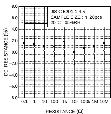
Fig.5 Resistance
