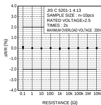
Fig.7 Overload
