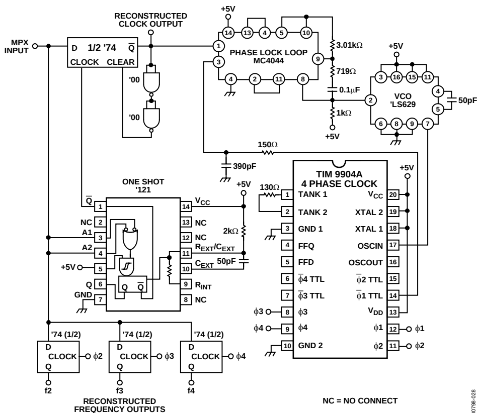
Figure 30. SVFC Demultiplexers
