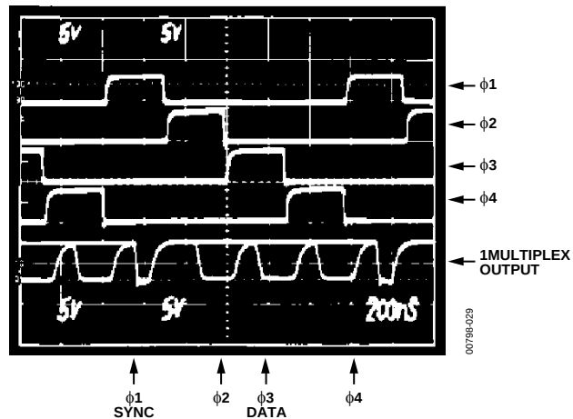
Figure 28. Multiplexer Waveforms
