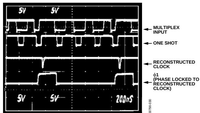
Figure 29. Demultiplexer Waveforms
