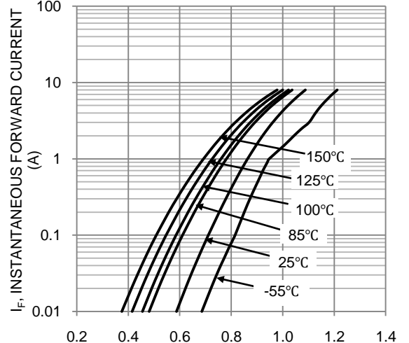
V_F , INSTANTANEOUS FORWARD VOLTAGE (V) Fig. 2 Typical Forward Characteristics (Per Leg)
