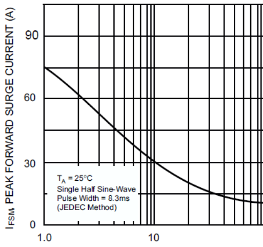
I_{FSM} , PEAK FORWARD SURGE CURRENT (A) NUMBER OF CYCLES AT 60 Hz Fig. 3 Maximum Peak Forward Surge Current (per leg)
