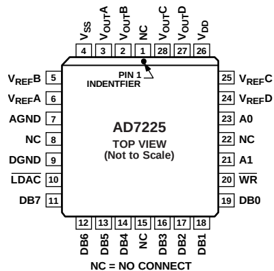
Figure 3. PLCC
