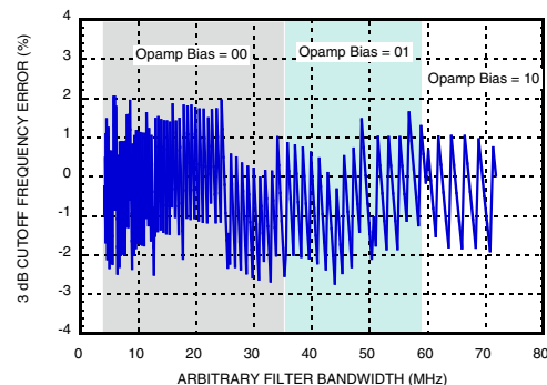
Figure 11. Arbitrary Bandwidth Setting 3 dB Cutoff Frequency Error [5]
