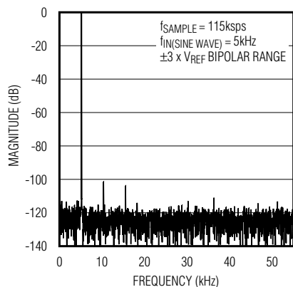
FFT AT 5kHz
