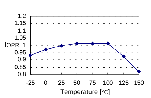
Figure 3. Operating Current
