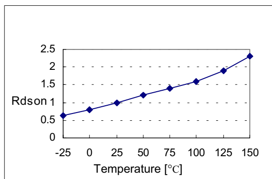
Figure 13. Drain Source Turn-on Resistance
