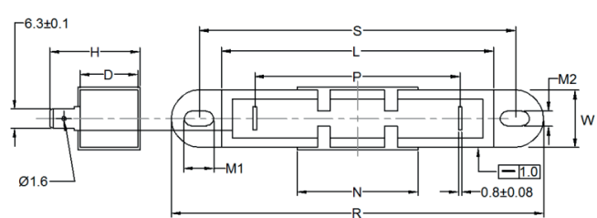
Figure 4 - quick connect "amp" tag with rugged bracket (AR)
