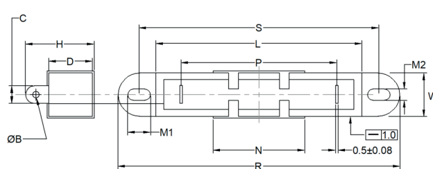
Figure 2 - soldered tag with rugged bracket (SR)
