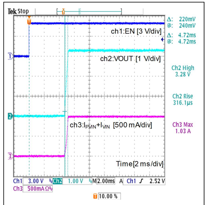
Figure 20. Startup Waveform (VIN=3.6 V, VSEL=High, MODE=High: Forced-PWM, 3.3 \Omega resistive load)
