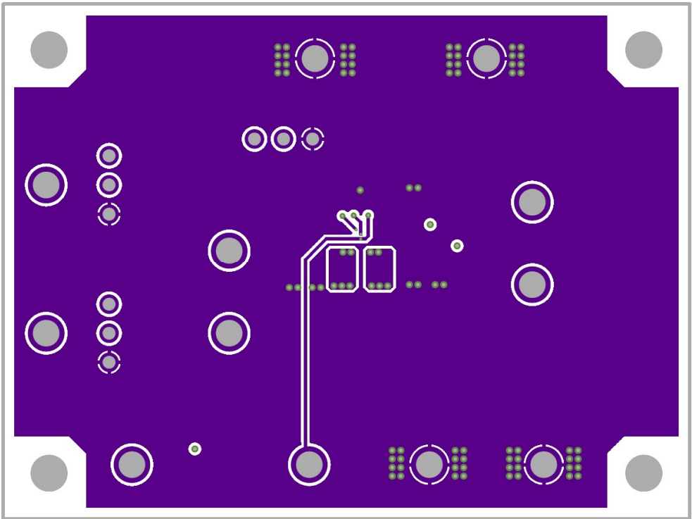
Figure 4. Middle 1 Layer
