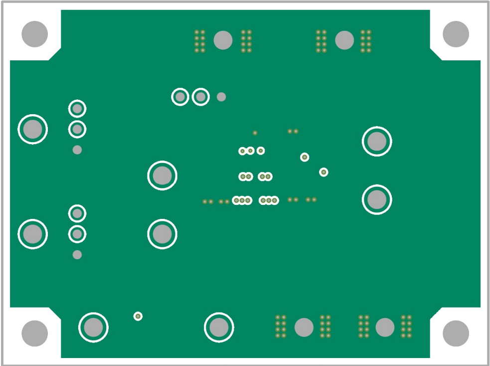
Figure 5. Middle 2 Layer
