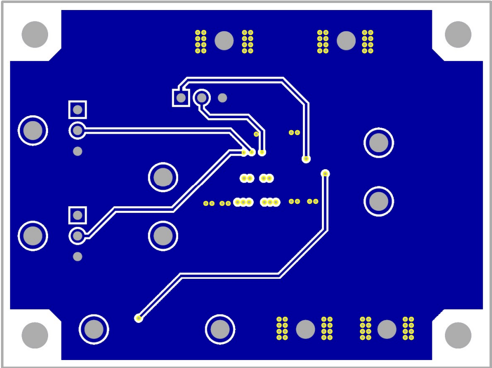
Figure 6. Bottom Layer
