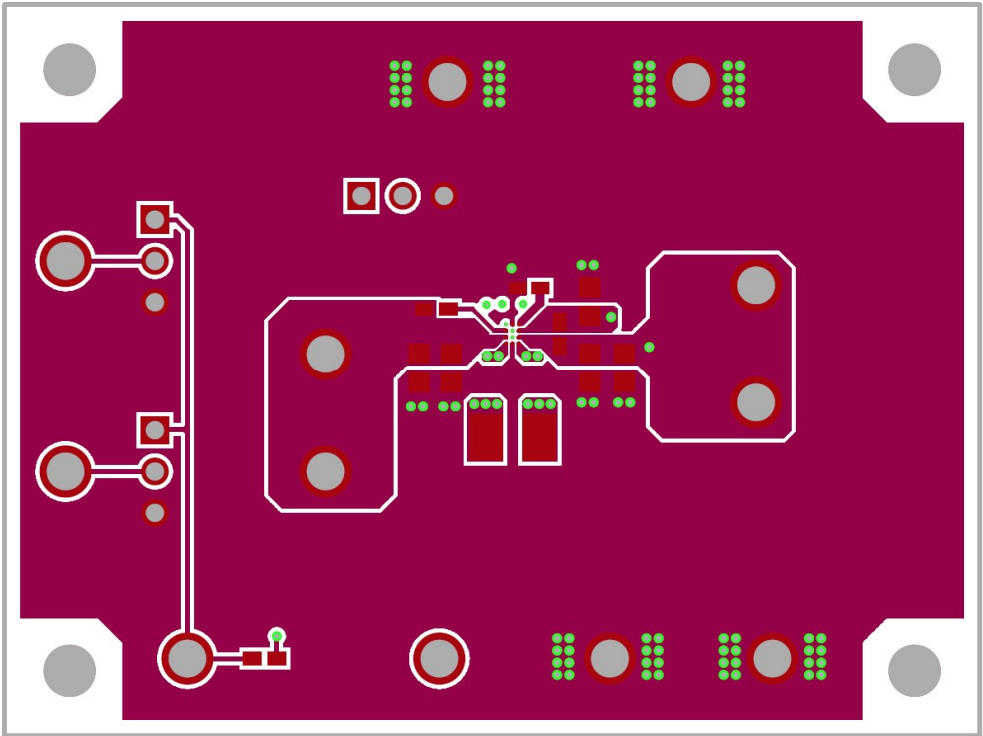
Figure 3. Top Layer
