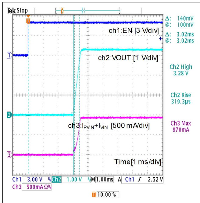
Figure 19. Startup Waveform (VIN=2.4 V, VSEL=High, MODE=High: Forced-PWM, 5.5 \Omega resistive load)
