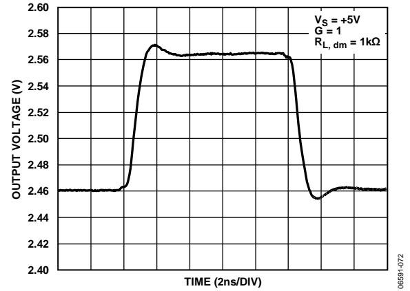
Figure 39. Small Signal V_{OCM} Pulse Response
