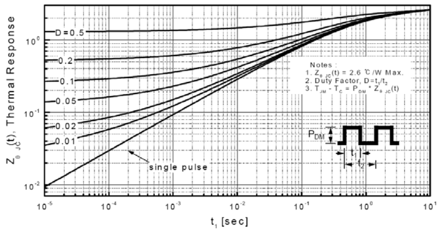
Transient Thermal Response Curve For JCS7N65FB
