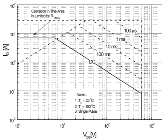
Maximum Safe Operating Area For JCS7N65FB
