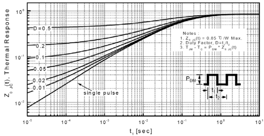
Transient Thermal Response Curve For JCS7N65FB
