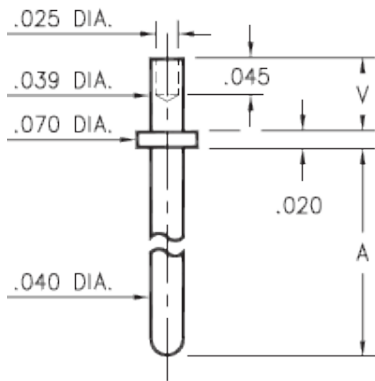
31XX-X-00-XX-00-00-08-0 Swage mount in .043 hole
