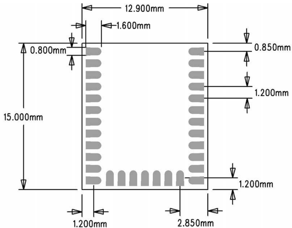
Figure 8.3. BGX13P Footprint
