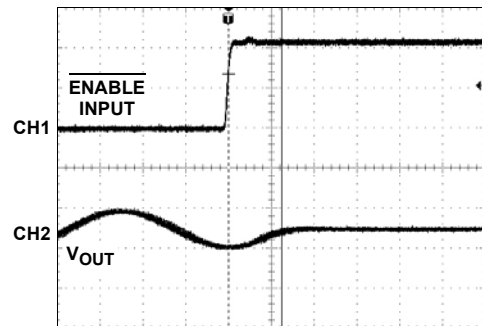
FIGURE 28. DISABLED RESPONSE
