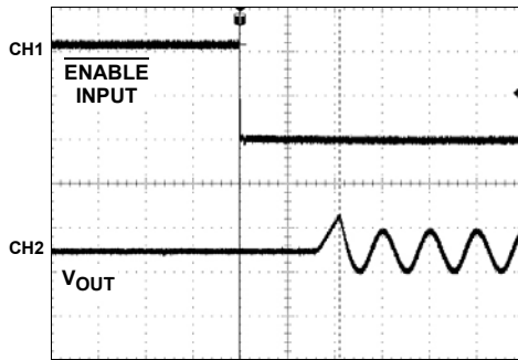
FIGURE 27. ENABLED RESPONSES
