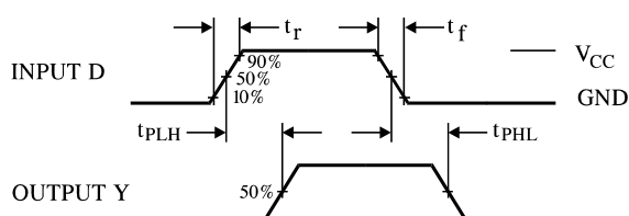
Figure 1. Switching Waveforms
