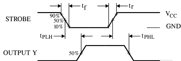
Figure 4. Switching Waveforms
