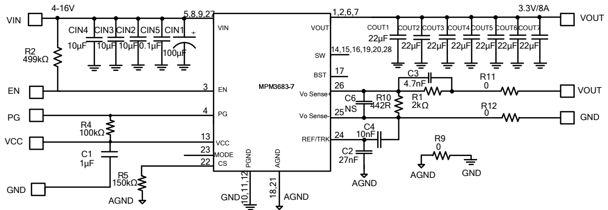
Figure 8: 12V IN 3.3V/8A Output
