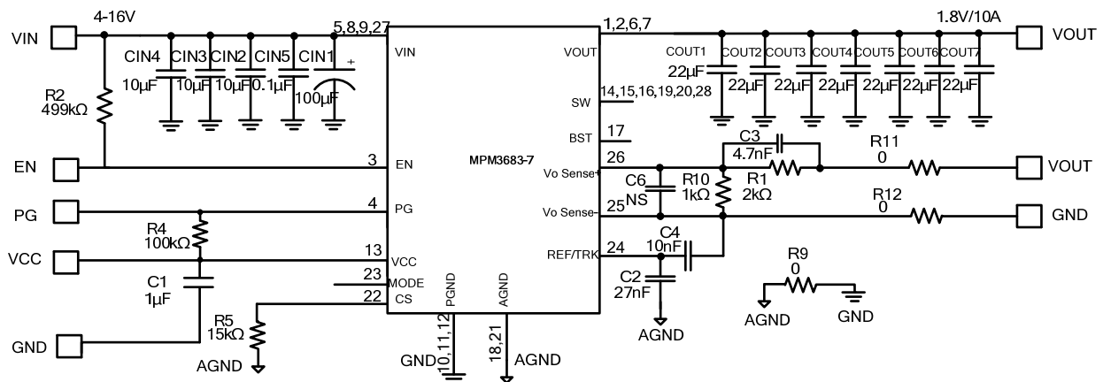
Figure 9: 12V IN 1.8V/10A Output
