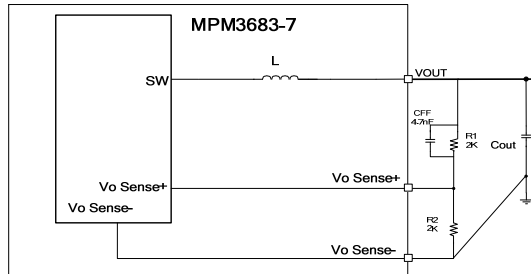
Figure 6: Circuit Connection
