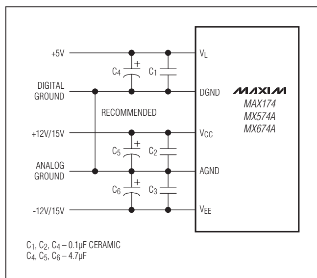
Figure 9. Power-Supply Bypassing
