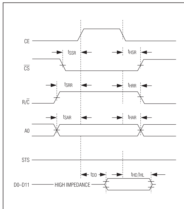
Figure 5. Read Timing
