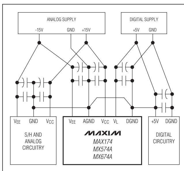
Figure 8. Power-Supply Grounding Practice
