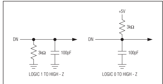
Figure 2. Load Circuit for Output Float Delay Test
