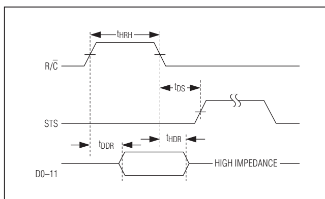
Figure 7. High Pulse for R/\overline{C} in Stand-Alone Mode
