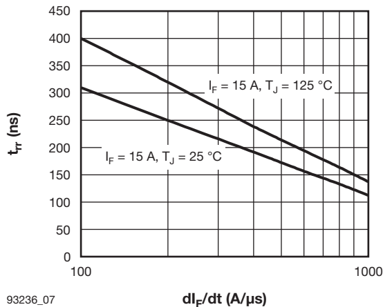
di_F/dt (A/ \mu s) Fig. 7 - Typical Reverse Recovery Time vs. di_F/dt
