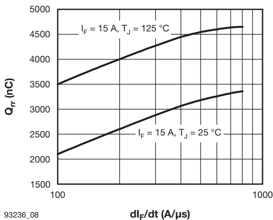
di_F/dt (A/ \mu s) Fig. 8 - Typical Stored Charge vs. di_F/dt
