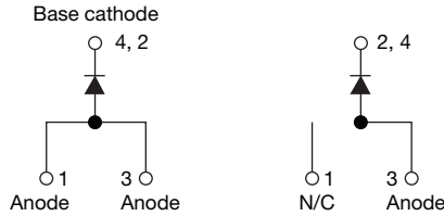
D-PAK (TO-252AA)
