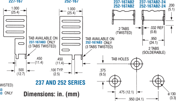
237 AND 252 SERIES Dimensions: in. (mm)
