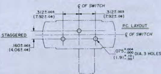
P.C. LAYOUTS (Top View)
