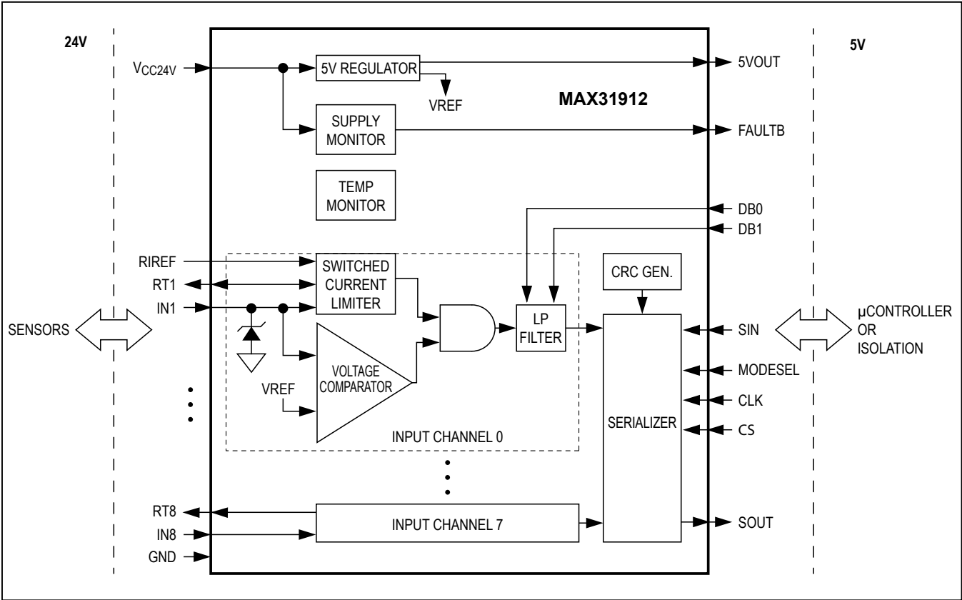
Block Diagram
