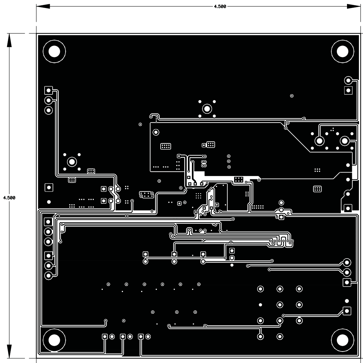
Figure 5. Third Layer
