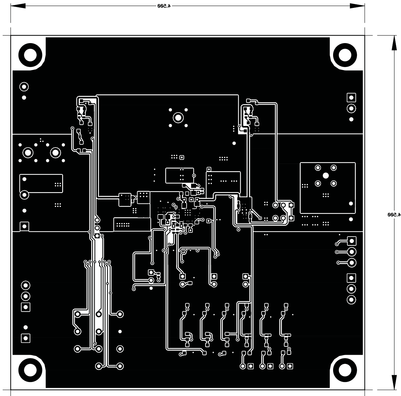
Figure 6. Bottom Layer
