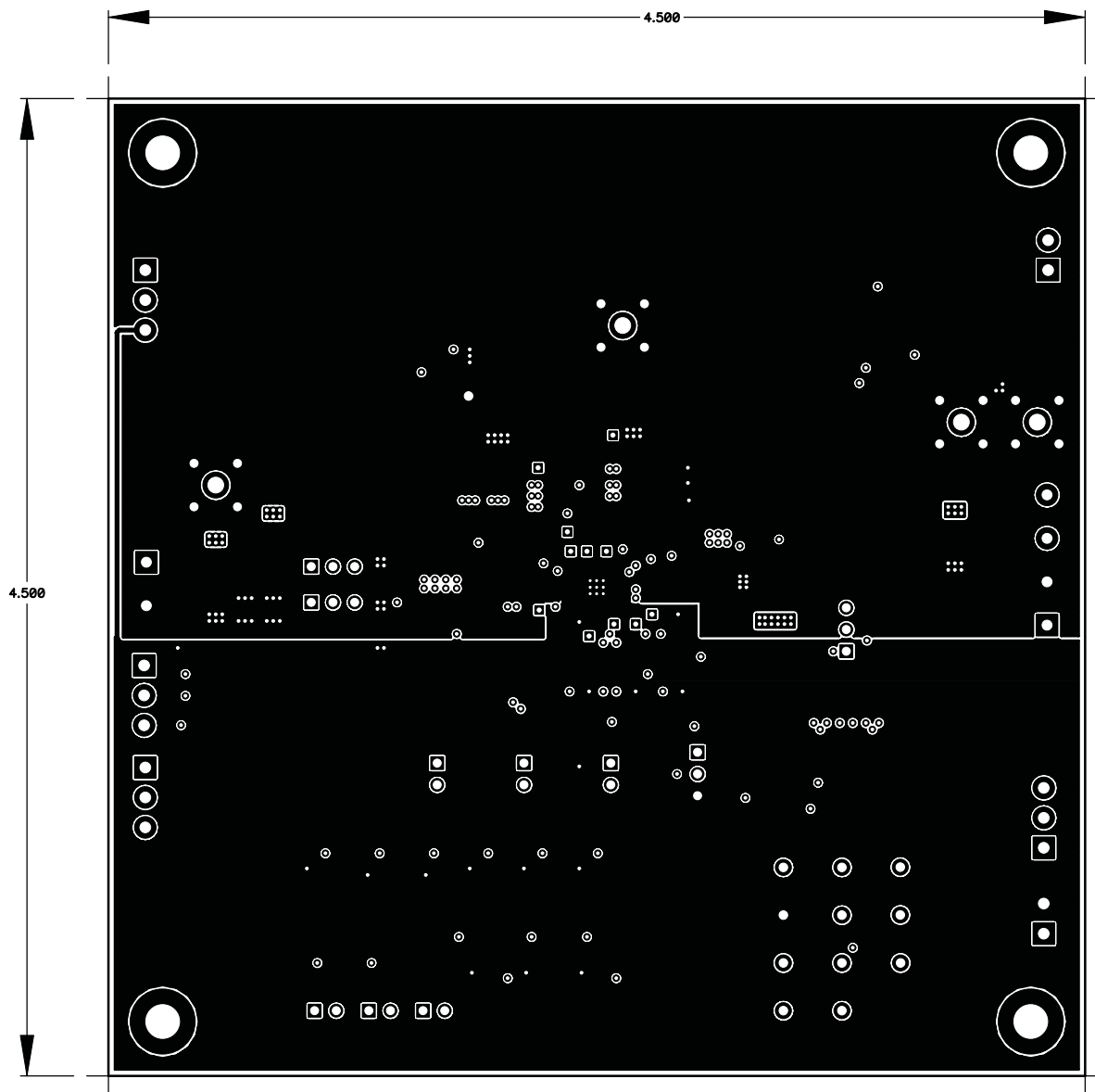
Figure 4. Second Layer
