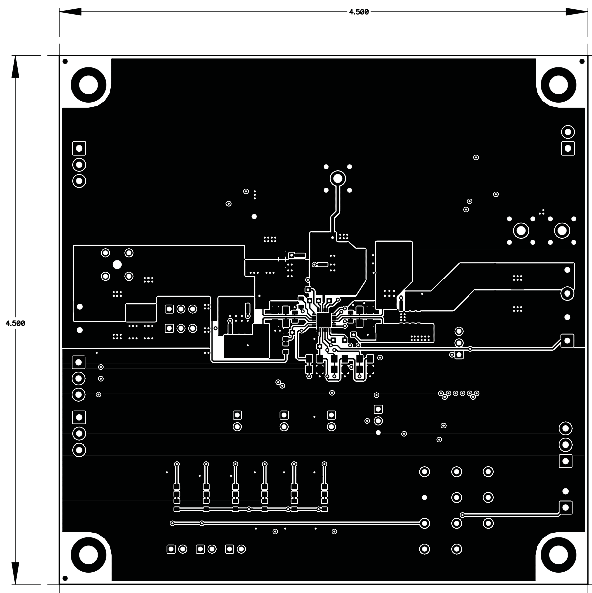
Figure 3. Top Layer
