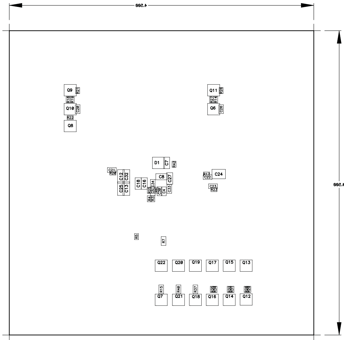
Figure 7. Bottom Assembly
