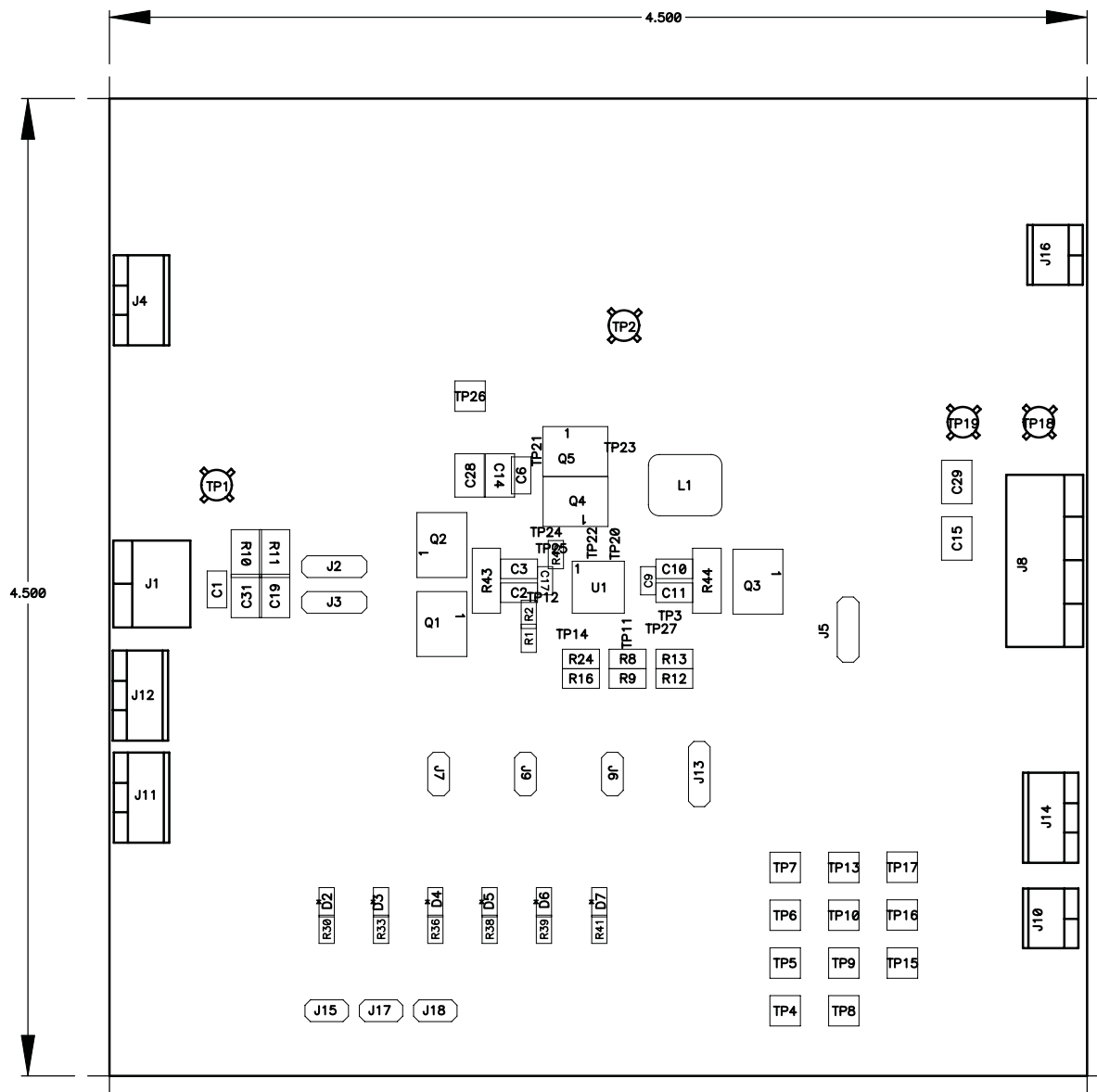
Figure 8. Top Assembly
