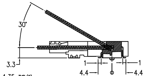
SECT X-X
