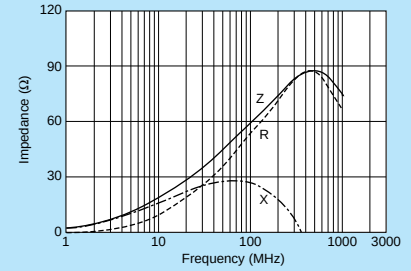
BLM21PG600SN1
