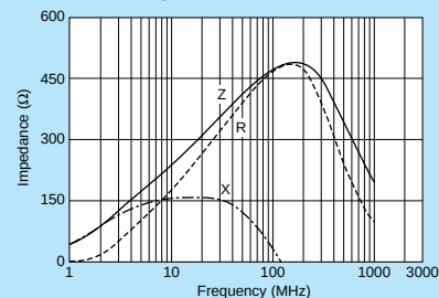
BLM21RK471SN1
