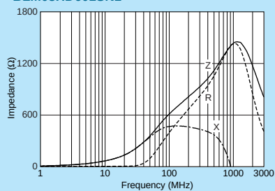
BLM03HD601SN1
