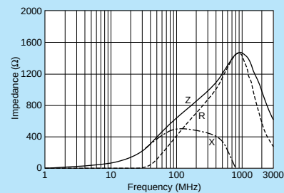
BLM15HD601SN1
