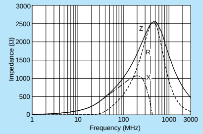
BLM18HD102SN1
