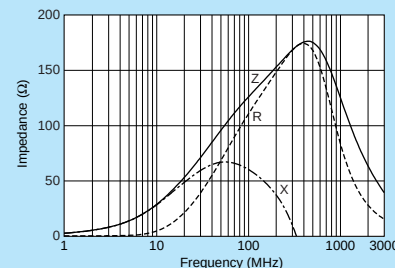
BLM15AG121SN1
