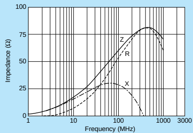
BLM41PG600SN1
