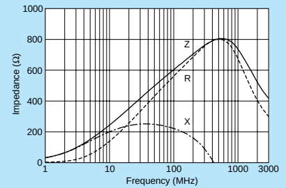
BLM18HK601SN1
