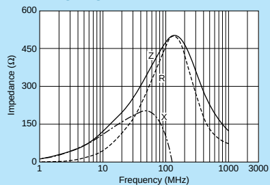
BLM41PG471SN1
