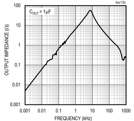
OUTPUT IMPEDANCE vs. FREQUENCY ( V_{OUT} = 4.096V )
