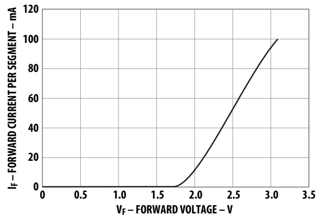
Figure 14. Forward current vs. forward voltage.
