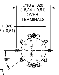
Terminal Detail
