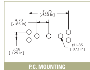
P.C. MOUNTING
