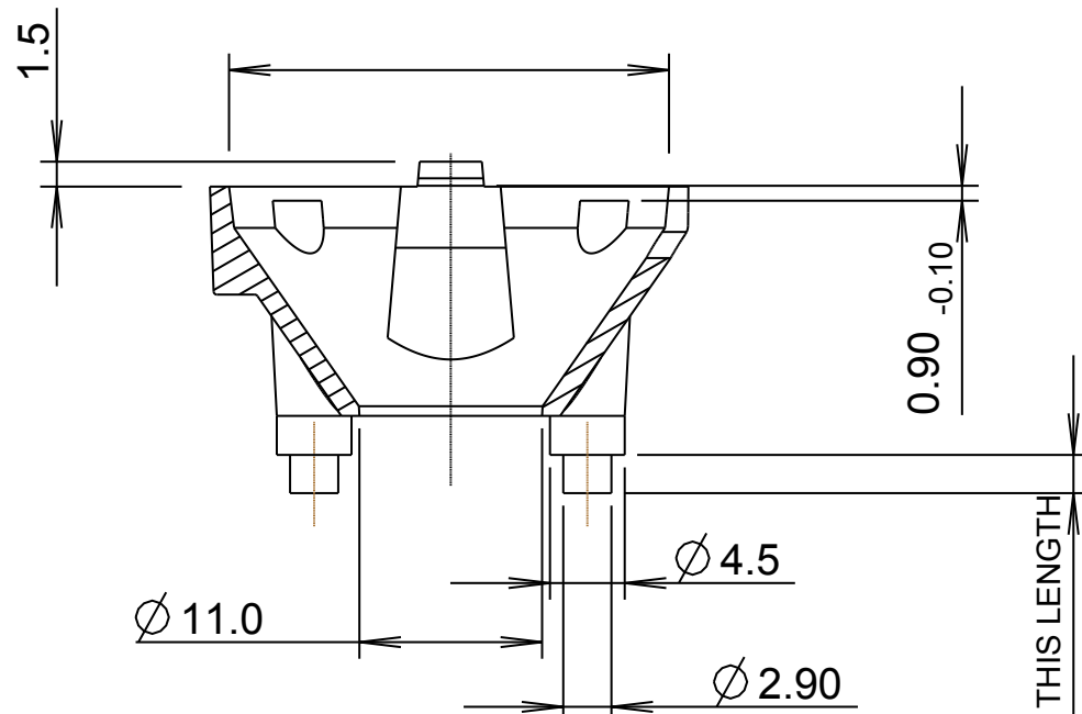
SECTION X-X
