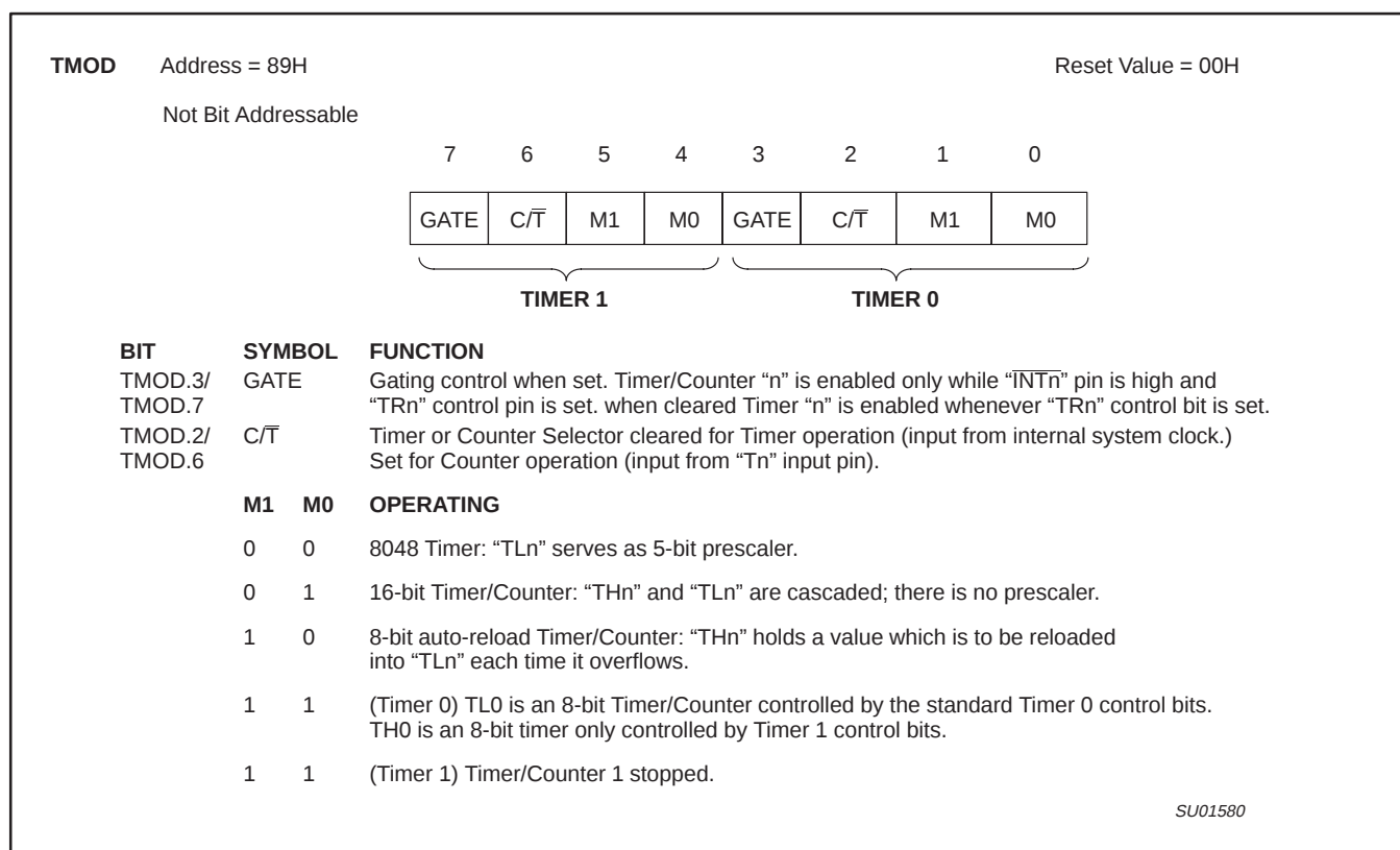
Figure 15. Timer/Counter 0/1 Mode Control (TMOD) Register
