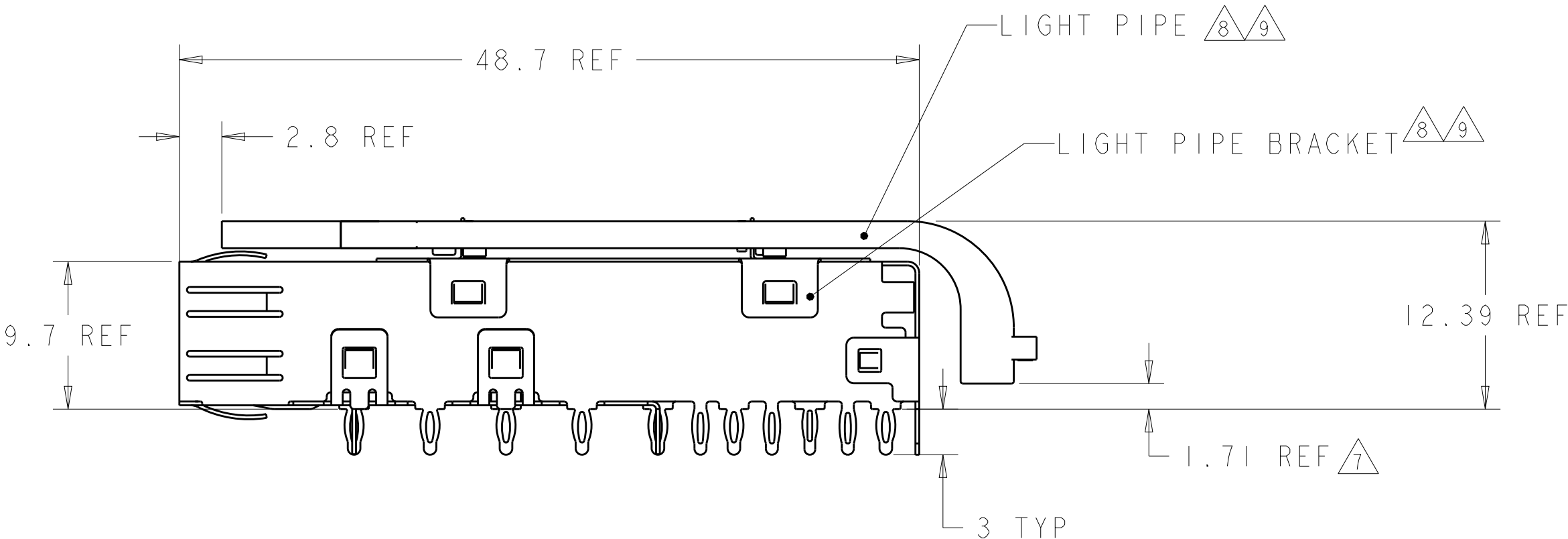
CAGE ASSEMBLY
