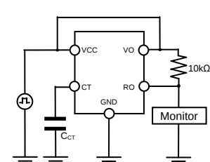
Measurement circuit for Figure.17, 18
