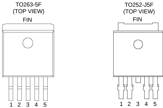
Figure 3. Pin configurations
