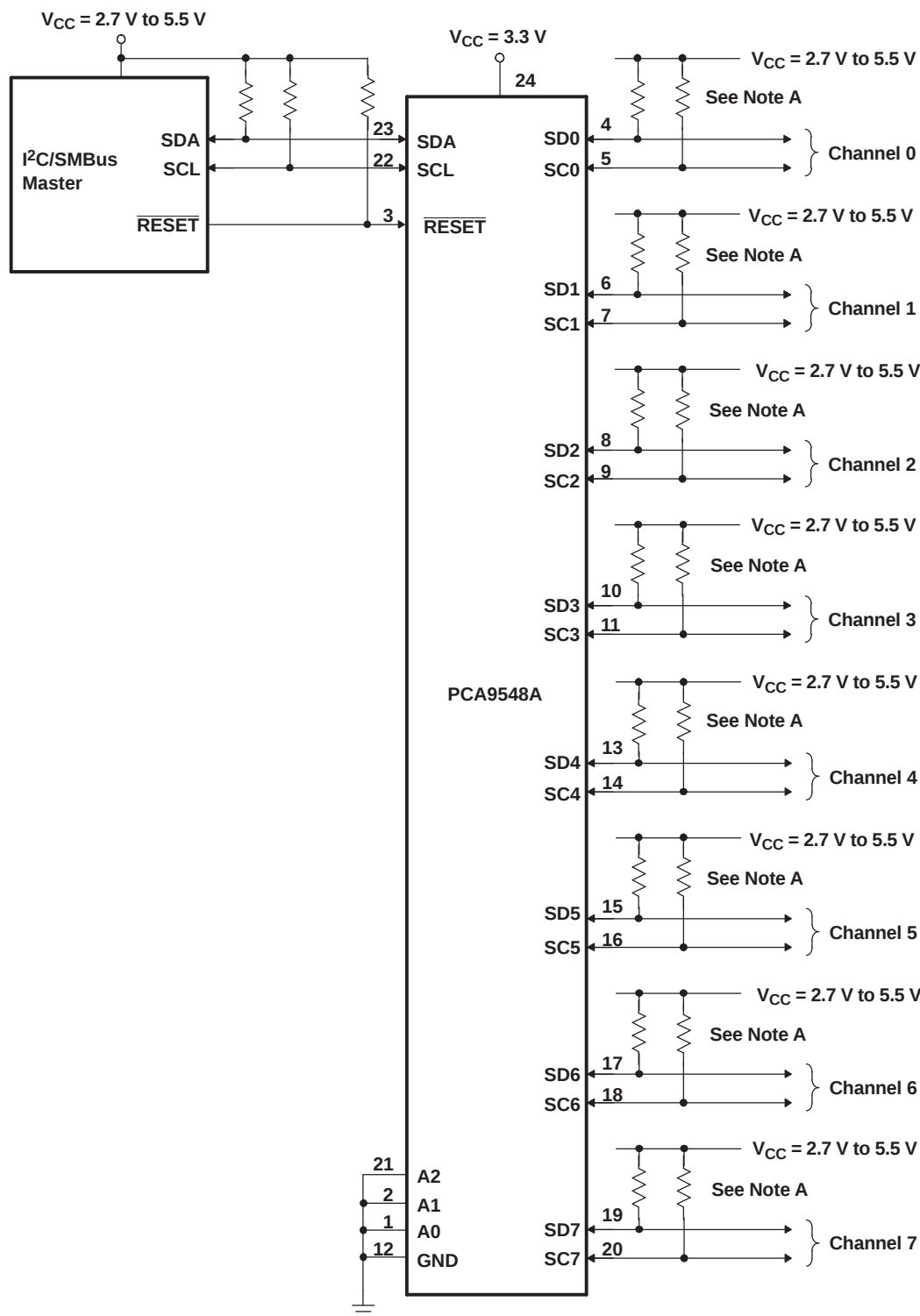
Figure 11. Typical Application
