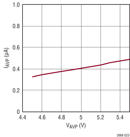
AVP Shutdown Current vs AVP
