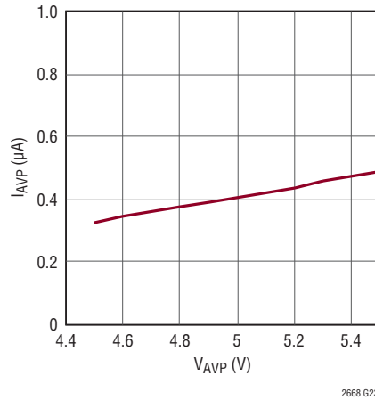
AVP Shutdown Current vs AVP
