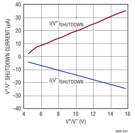
V + /V - Shutdown Current vs Symmetric Supplies
