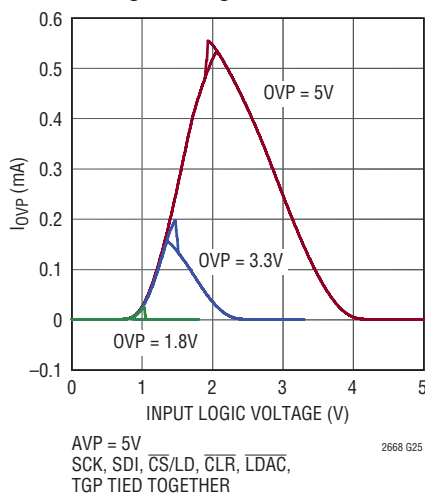
IOVP Supply Current vs Logic Voltage
